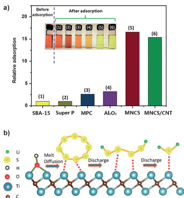
Figure 2. a) The relative adsorption amounts (normalized to the value of Super P carbon black) of MNCS compared with other adsorbents. Inset: Photographs of polysulfide solutions before and after adsorption. [9] b) Representation of S–Ti–C bond formation on the MXene (Ti 2 C) surface. [10] SBA-15 is a form of mesoporous silica. MPC = mesoporous carbon.
